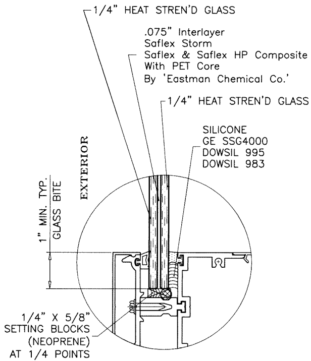
GLASS TYPE 'A' LEVEL 'D' IMPACT
