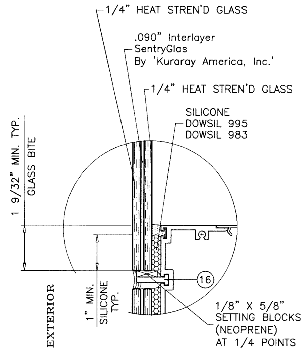
GLASS TYPE 'C' LEVEL 'D' IMPACT
