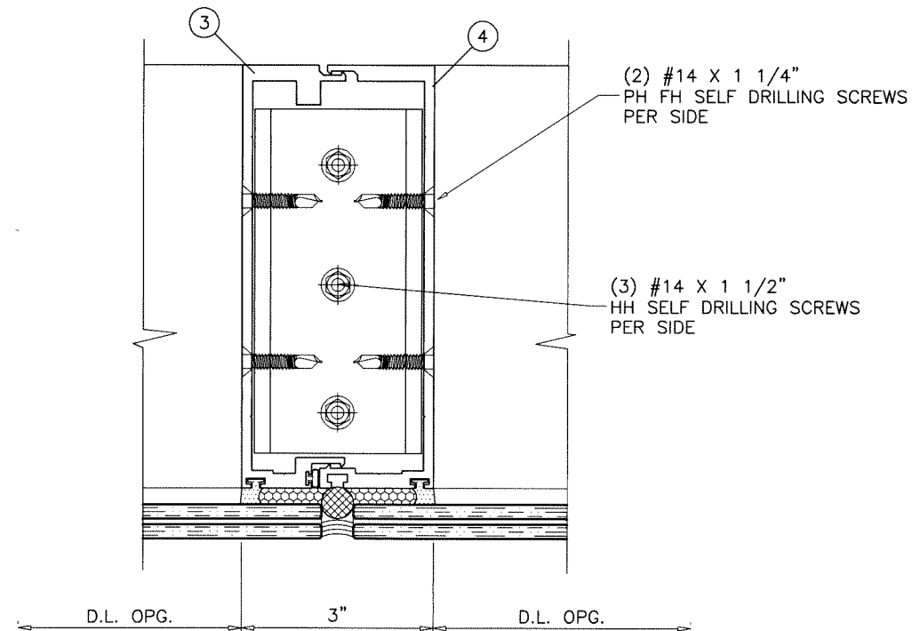
DETAIL '4' AT MULLION ABOVE DOOR
