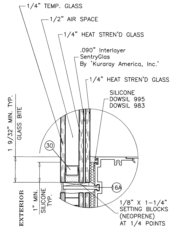
GLASS TYPE 'C1' LEVEL 'D' IMPACT
